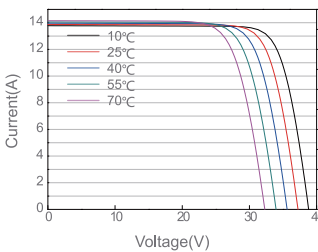
Current-Voltage Curve JAM108S-405
