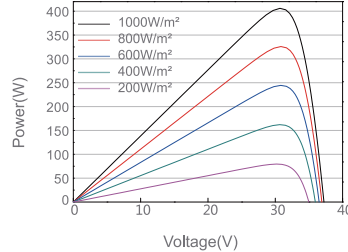
Power-Voltage Curve JAM108S-405
